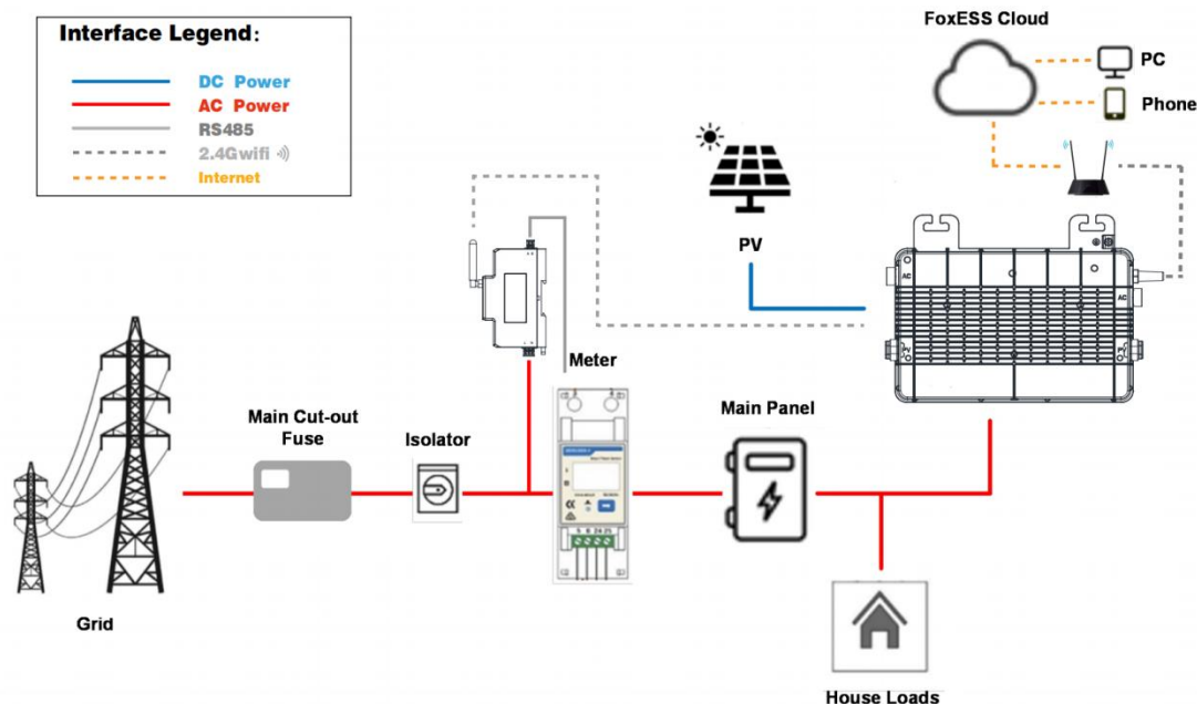
Figure 1 The system diagram with SMART GW control for micro inverter.
